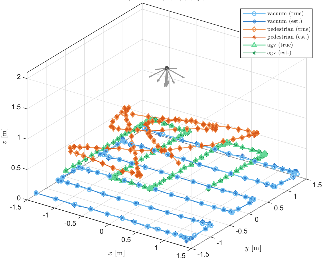
Broadcast 3D Positioning: 3 Simultaneous Users
