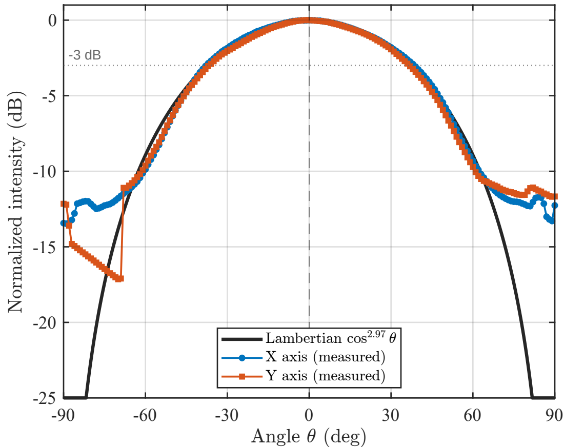
LED radiation pattern: X/Y axes vs. Lambertian ( m = 2.97 )
