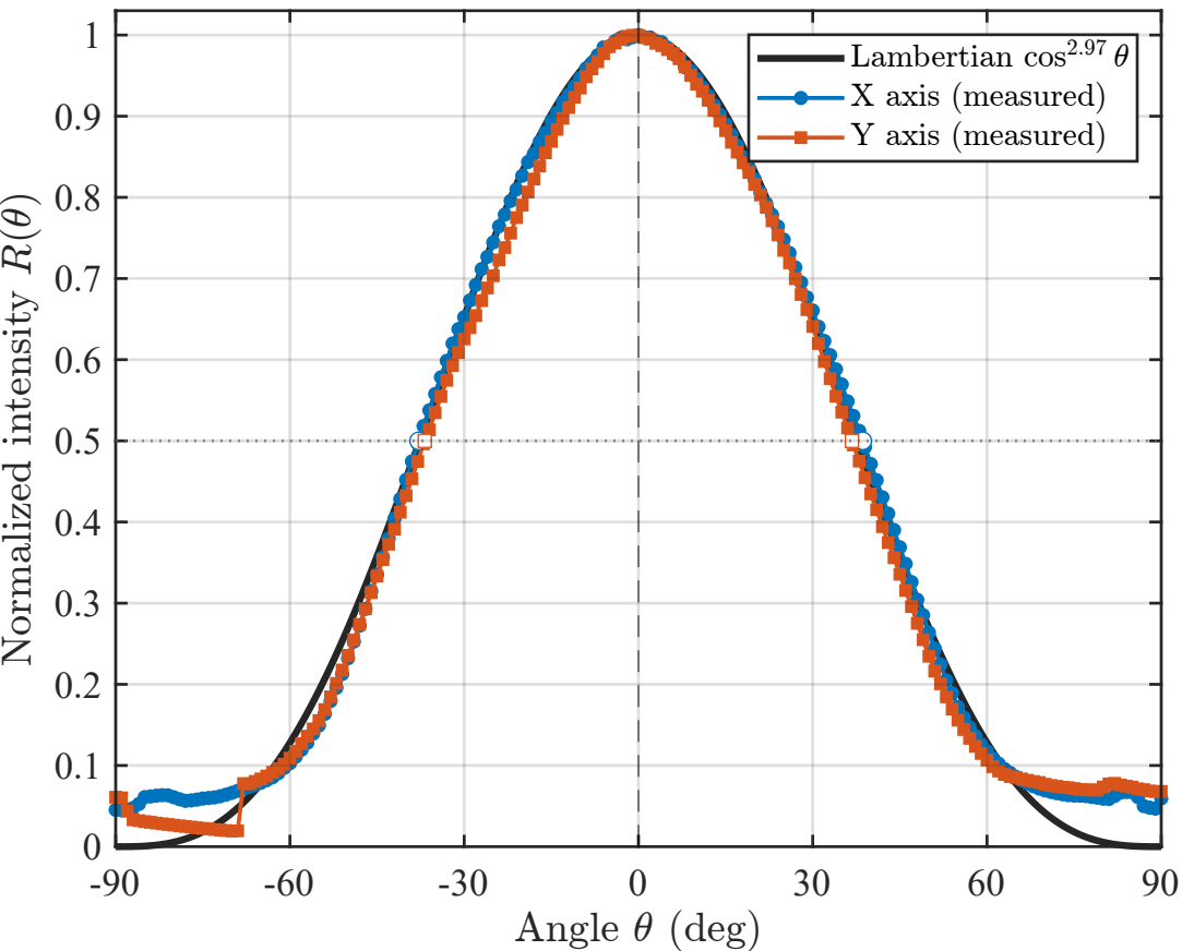
LED radiation pattern: X/Y axes vs. Lambertian ( m = 2.97 )
