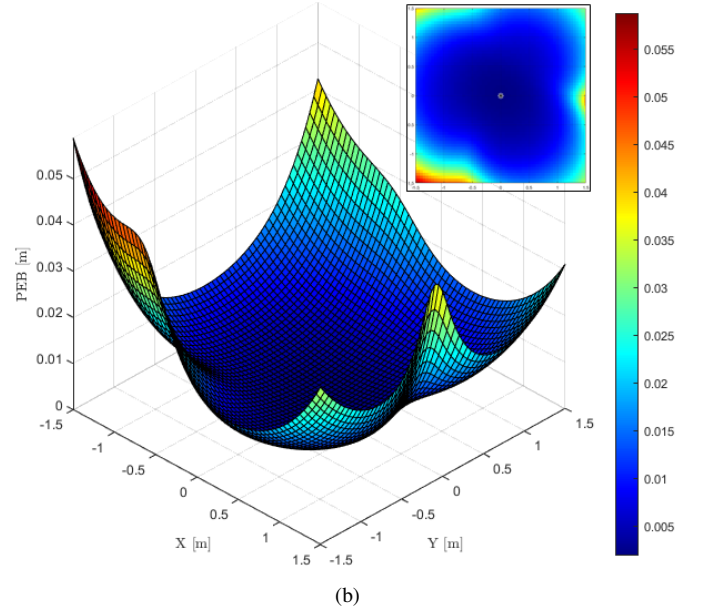
Fig. 3. Heat map of the PEB across a 3 \times 3 \text{ m} testbed at z = 0.8 \text{ m} for K = 5 orientations: (a) optimal set, (b) sub-optimal set.
