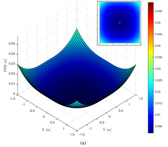
Fig. 2. RMS performance in a 3 \times 3 \text{ m} testbed using an optimal set of K orientations versus a sub-optimal set of K orientations.
