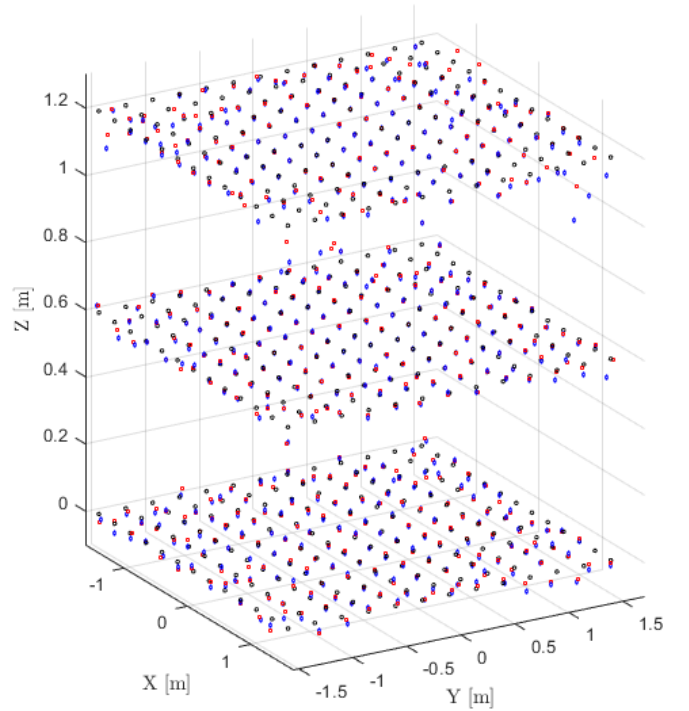
Fig. 8. 3D position estimates at three receiver heights for K = 5 orientations: GLS (blue), WLS (red), true positions (black).
