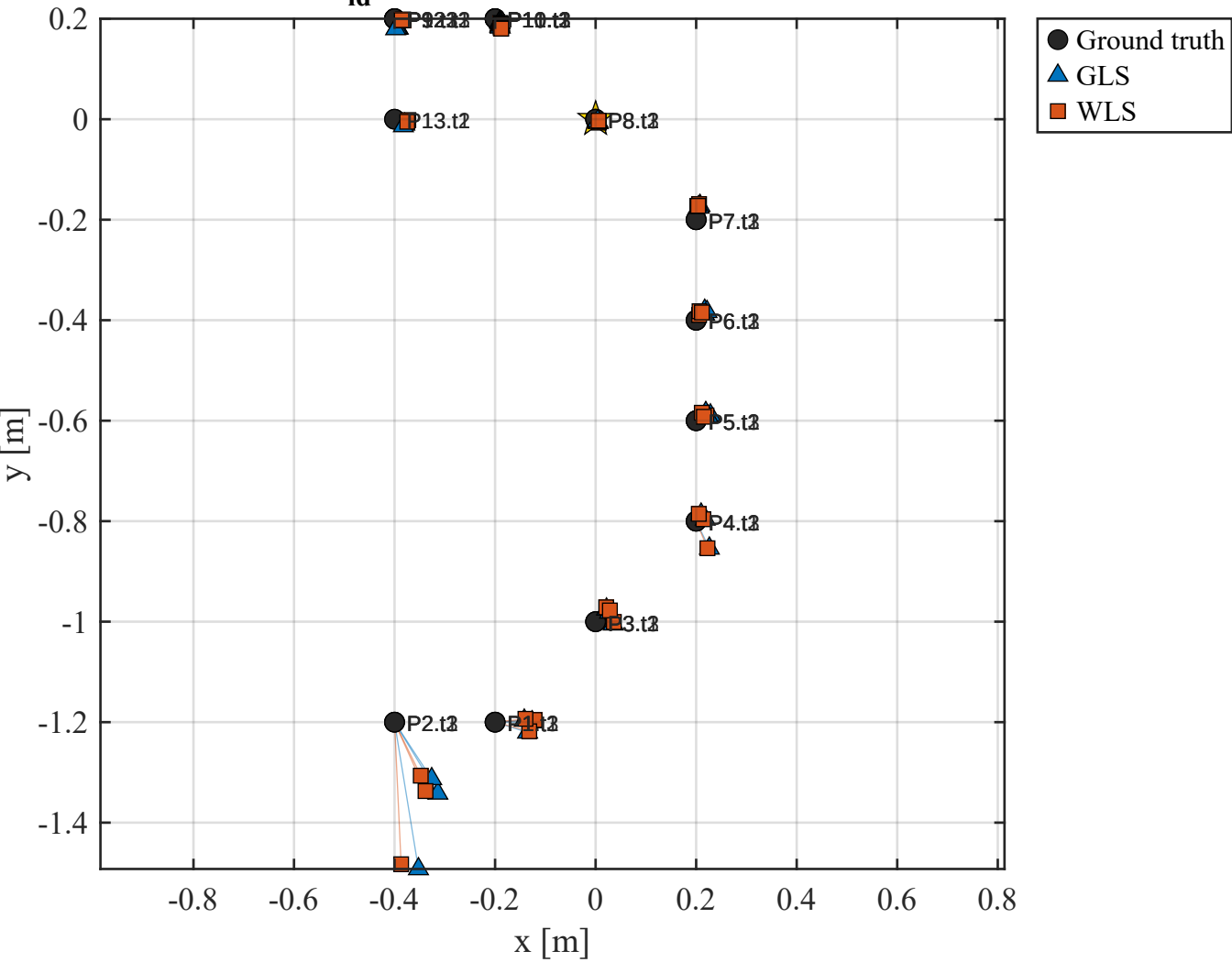
Top-view localization (X-Y) tilt PD | K_{id}=[1\ 2\ 3\ 4\ 5\ 6\ 7\ 8\ 9\ 10\ 11\ 12] | m=3.13
