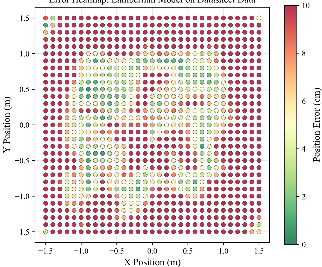
Error Heatmap: Lambertian Model on Datasheet Data
