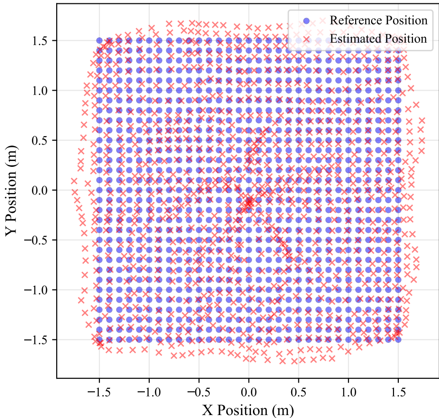
Cross-Model Test: Lambertian Model on Datasheet Data
