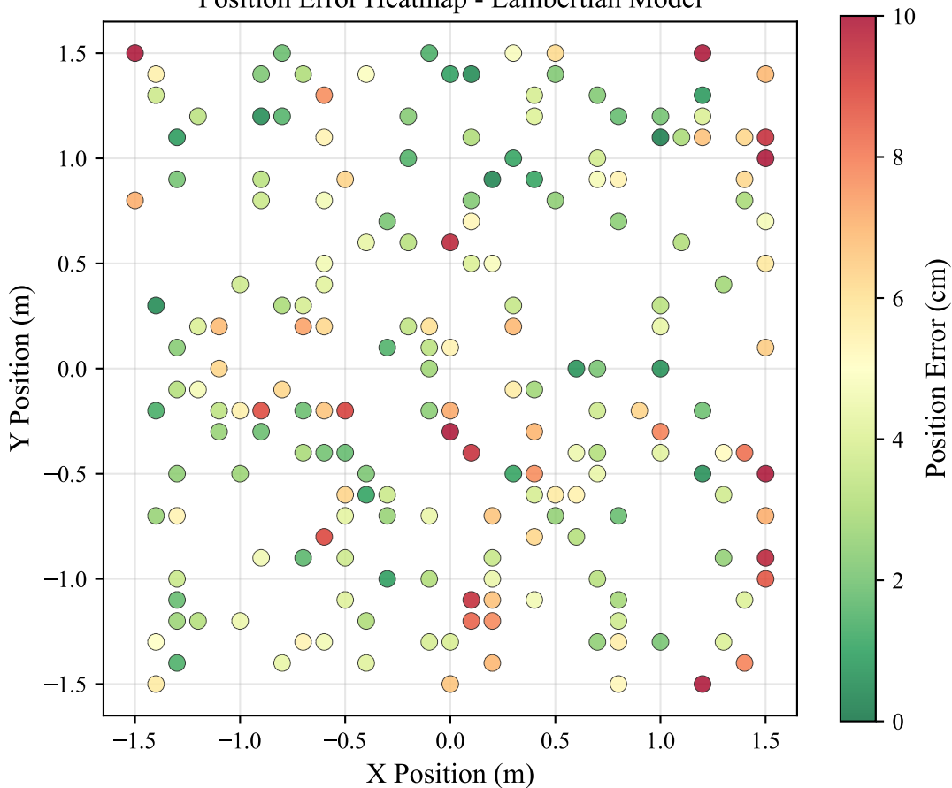
Position Error Heatmap - Lambertian Model
