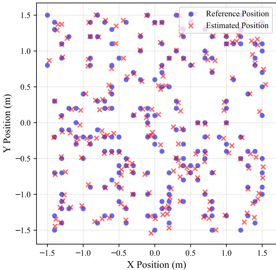
Position Estimation - Lambertian Model
