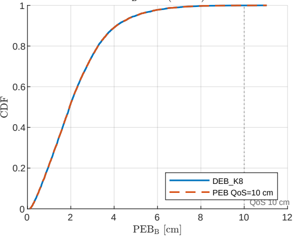
PEB B CDF ( K = 8 )
