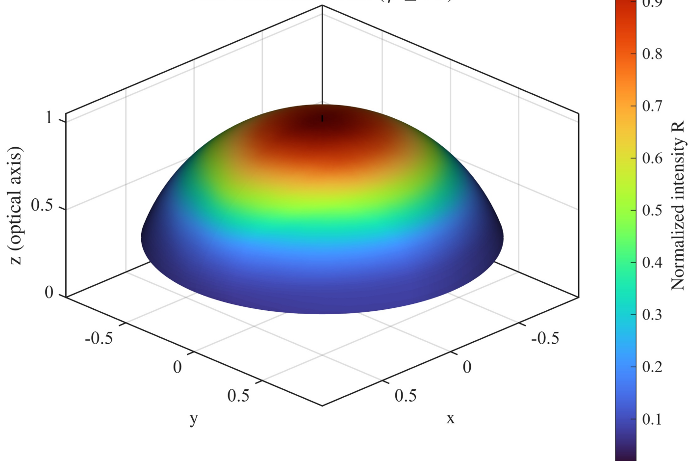
LED illumination cone ( \phi \leq 70^\circ )
