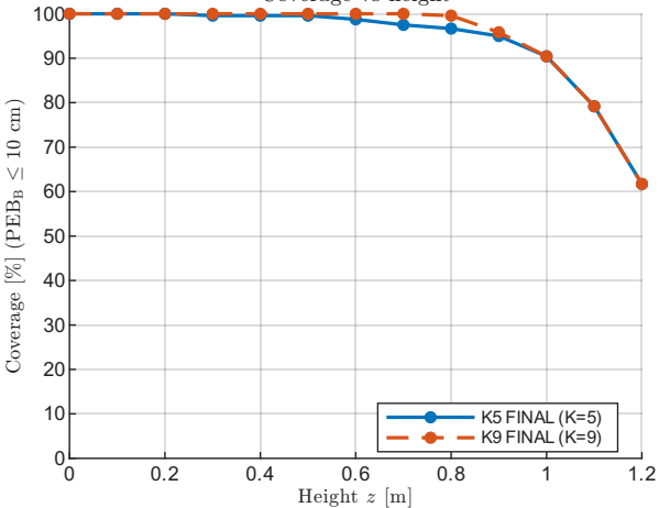
Coverage vs height
