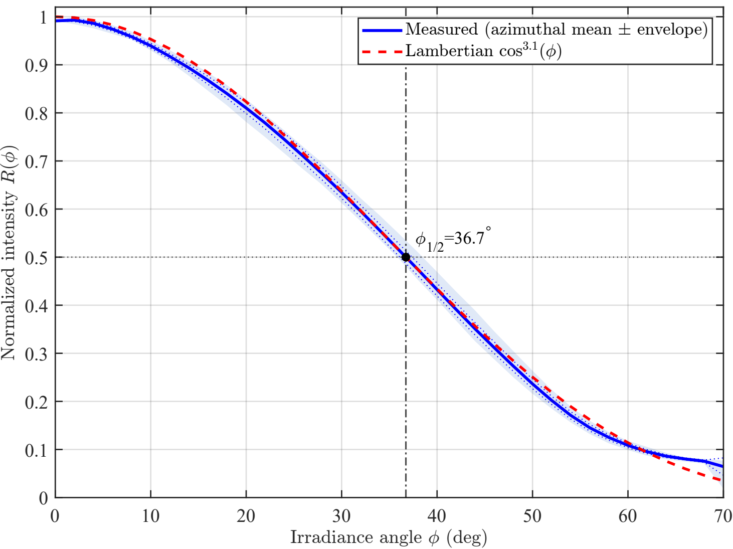
Measured radiometric profile vs. Lambertian model
