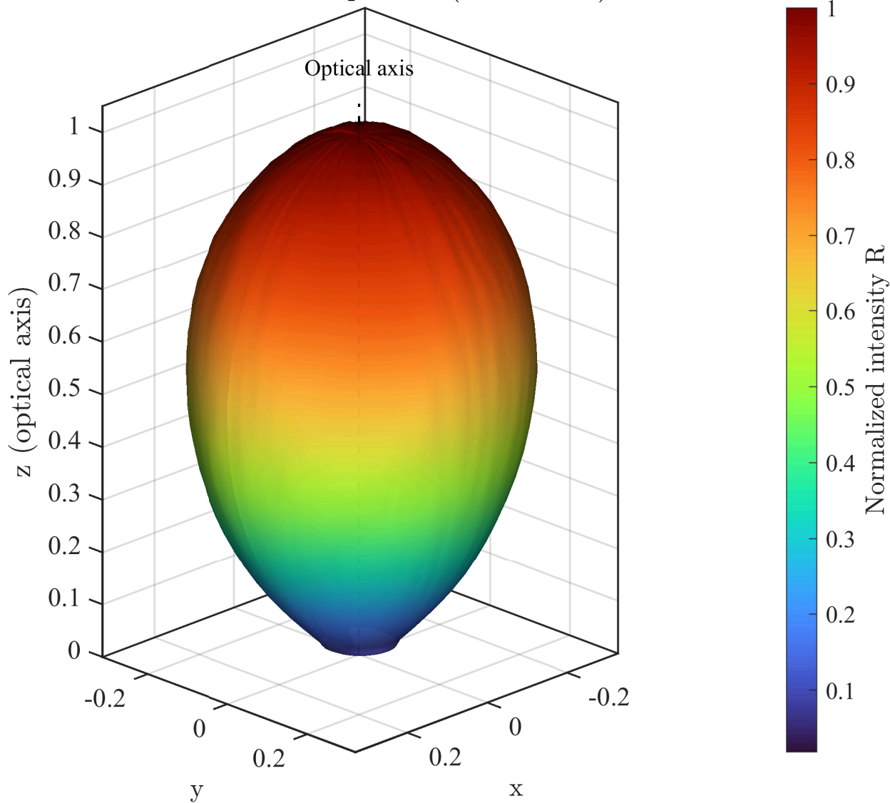
3D LED radiation pattern (radius = R )
