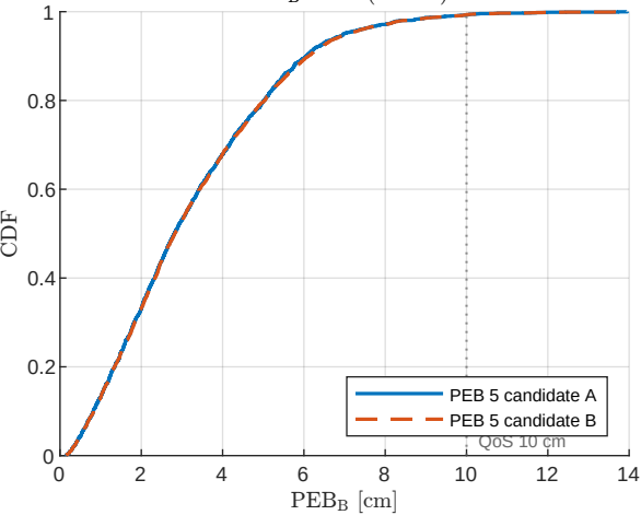
PEB B CDF ( K = 5 )
