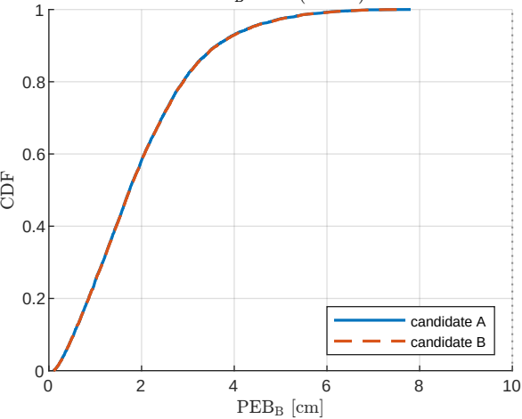
PEB B CDF ( K = 9 )
