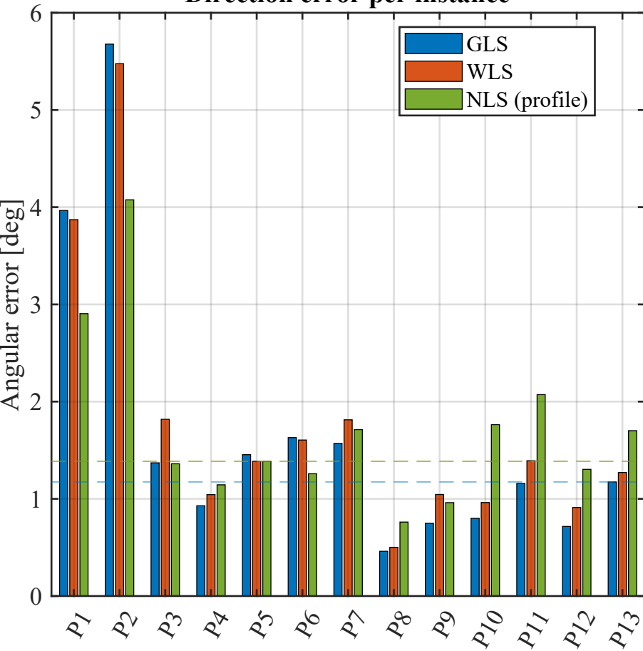
Direction error per instance
