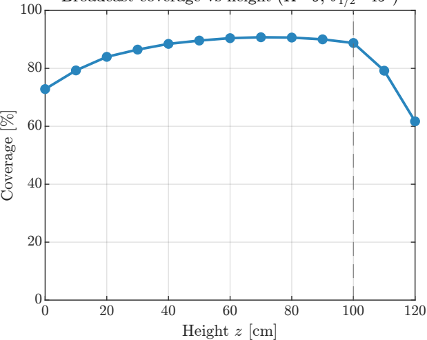
Broadcast coverage vs height ( K=9 , \theta_{1/2}=45^\circ )
