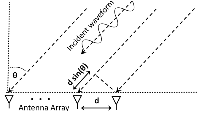
Fig. 2. AoA based localization.
