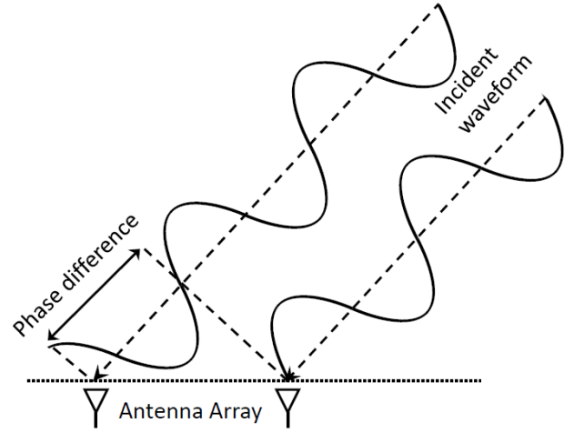
Fig. 5. PoA based localization.
