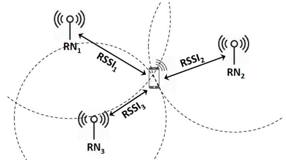
Fig. 1. RSSI based localization.
