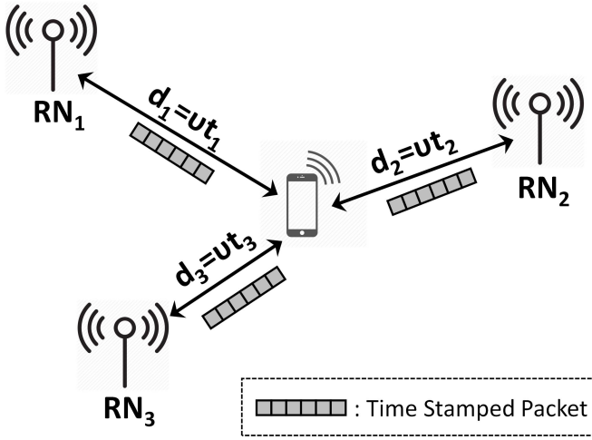
Fig. 3. ToF based user equipment (UE) localization.
