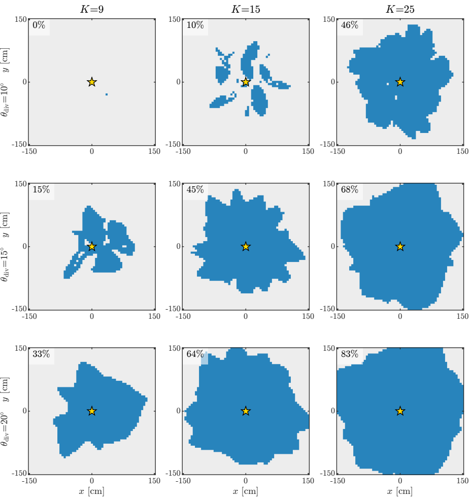
Localization coverage @ z = 0.8 m (blue = covered)
