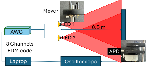
Fig. 2: Experiment set-up for ML-based OWP with the interference
