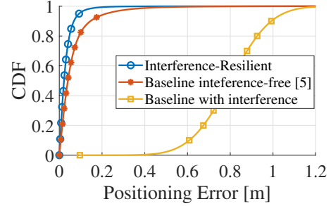
Fig. 4: Simulation for positioning error in CDF
