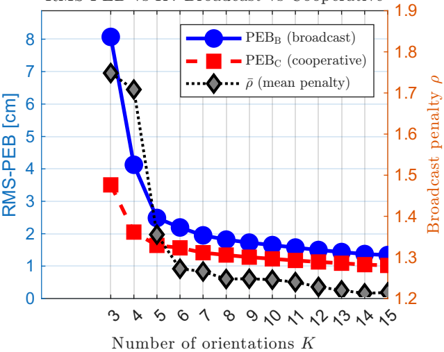
RMS-PEB vs K : Broadcast vs Cooperative
