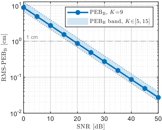
Broadcast PEB vs SNR ( \Phi_{1/2}=45^\circ , \mathbf{n}_r=[0, 0, 1]^T , DEB-opt.)
