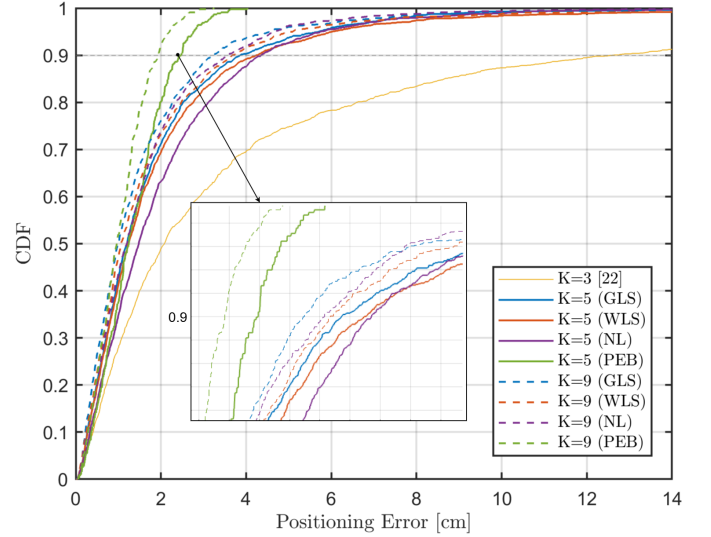
Fig. 6. Comparison of the CDFs of different 3D position estimation methods for K = 3, 5, 9 .
