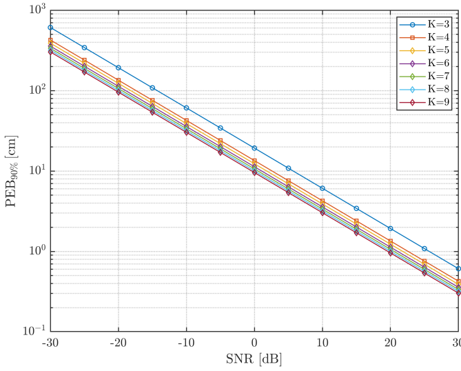
Fig. 5. \text{PEB}_{90\%} versus SNR for GA-optimized orientation sets with K \in \{3, \dots, 9\} ( \Phi_{1/2} = 45^\circ ; remaining parameters in Table ??). Values are computed over all receiver positions in the 3 \times 3 \times 2 \text{ m}^3 testbed.
