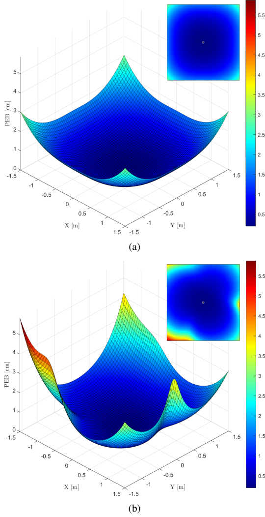
Fig. 3. Heat map of the PEB across a 3 \times 3 \text{ m}^2 testbed at z = 0.8 \text{ m} for K = 5 orientations: (a) optimal set, (b) random set.
