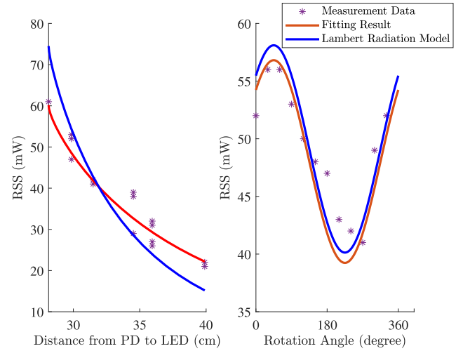
Fig. 23. Sampled RSS values, fitted curves, and Lambert radiation model for different distances and rotation angle values.
