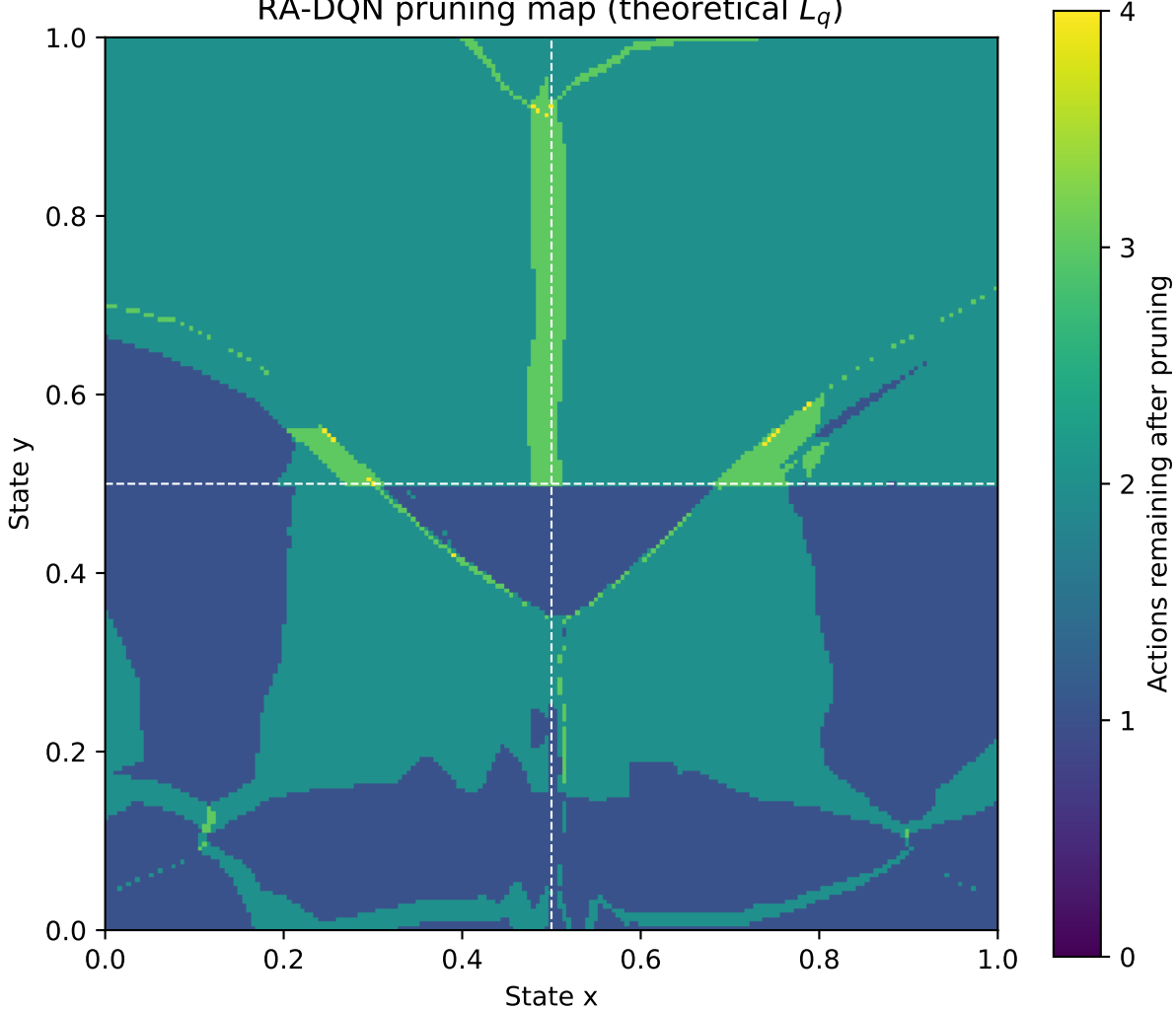
RA-DQN pruning map (theoretical L_q )
