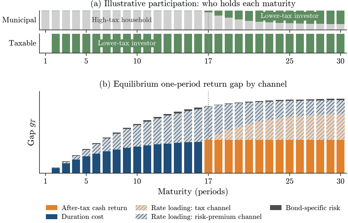
Figure 5: Participation and the equilibrium one-period return gap in a thirty-maturity two-investor illustration. The lower-tax investor holds municipal bonds from T^* = 17 (dotted vertical line). Panel (a) shows each investor's share of each municipal and taxable maturity at the mean state, an illustrative pattern that differs from participation in the calibrated economy (Section 6). The one-period taxable claim is cash. Panel (b) shows the gap g_T = \mu_T^M - \xi_H \mu_T^C at the mean state by channel, (43), with the rate loading hatched by response channel and the small bond-specific term on top. Shares and levels depend on illustrative parameters (Appendix A.10), so the panels omit vertical scales.
