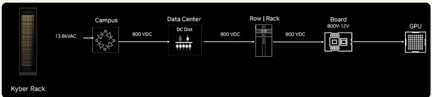
A figure showing the rack architecture for Kyber, designed for 800 VDC.
