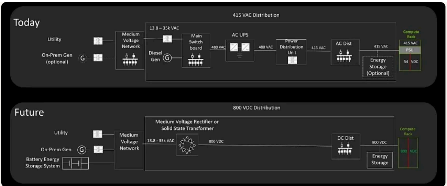
Figure showing today's power distribution versus the future.
