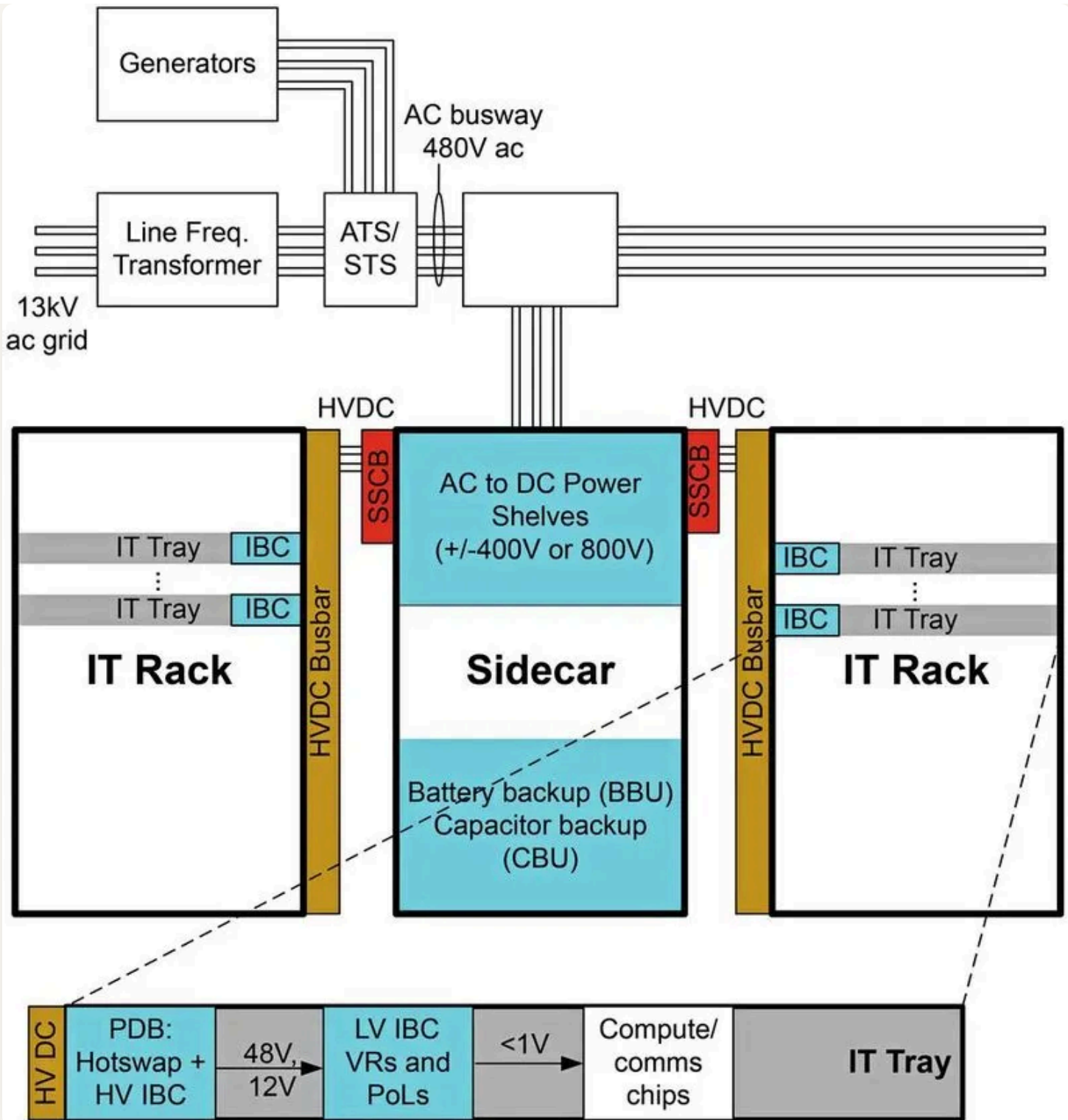
Sidecars: The New Power Supply Concepts for AI Data Centers
