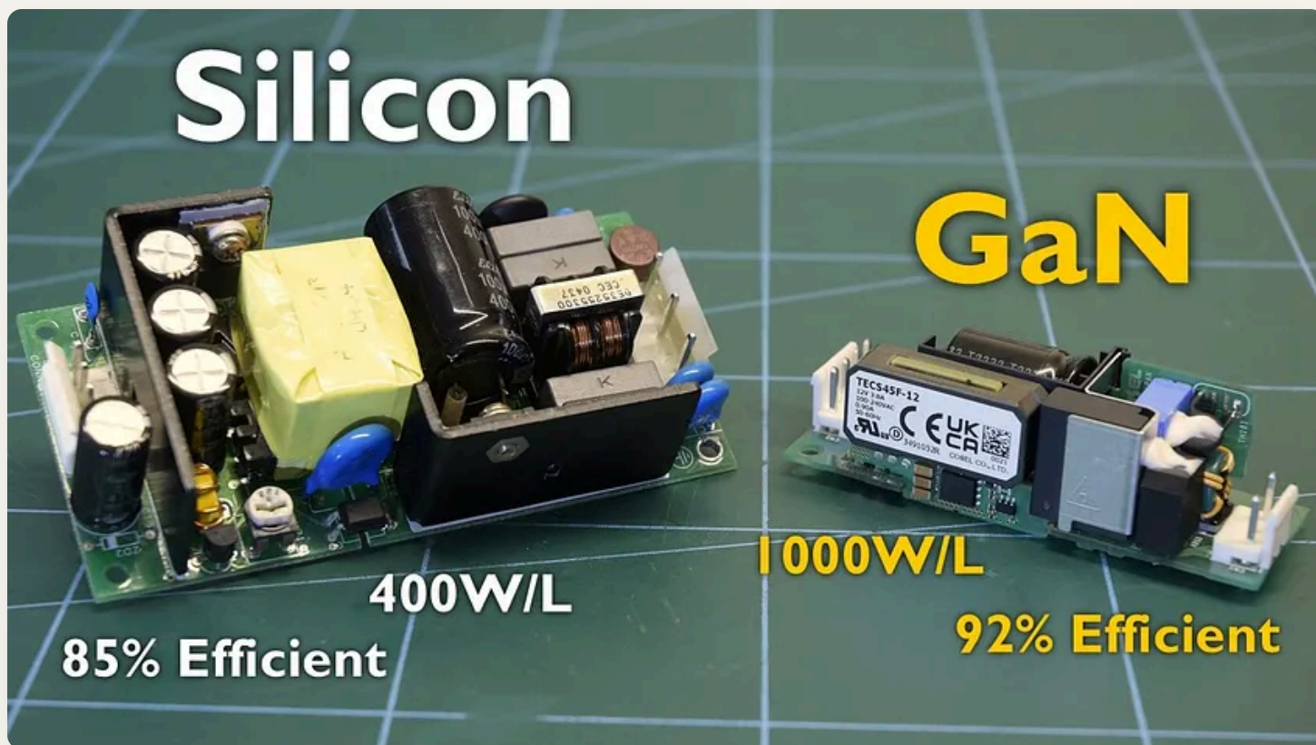
Everything is Better: GaN vs Silicon Power Supplies
