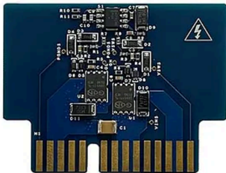
Discrete GaN
