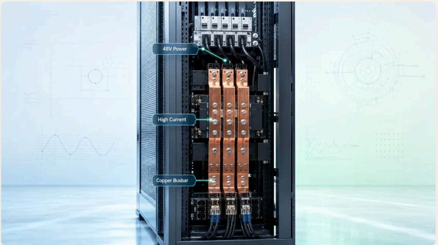
Bus Bar for Server Rack Power Distribution: What Data Center Buyers Should Know
