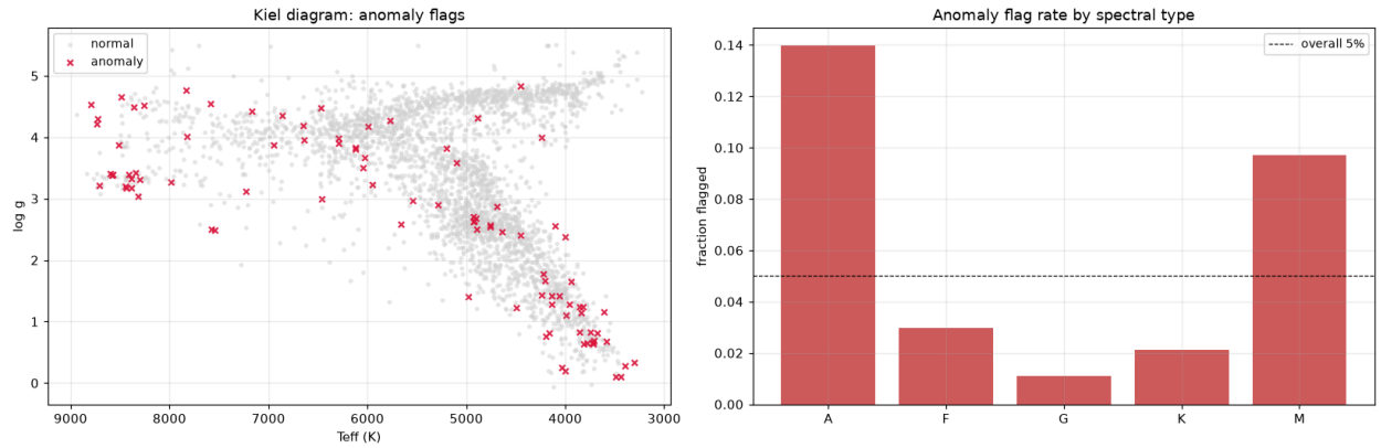
Figure 8.2.3: Anomaly flags overlaid on the Kiel diagram (left) and anomaly flag rate by spectral type relative to the overall 5% contamination threshold (right).
