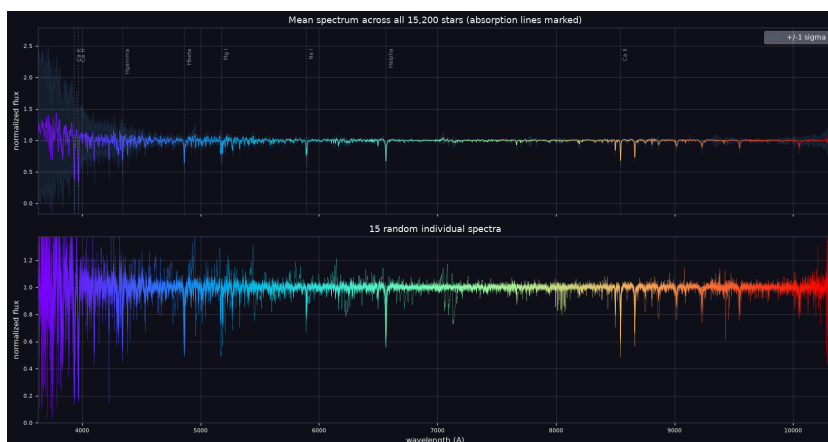
Figure 7.3: Mean continuum-normalized spectrum with \pm 1\sigma band and labeled absorption lines (top), and 15 randomly sampled individual spectra (bottom).
