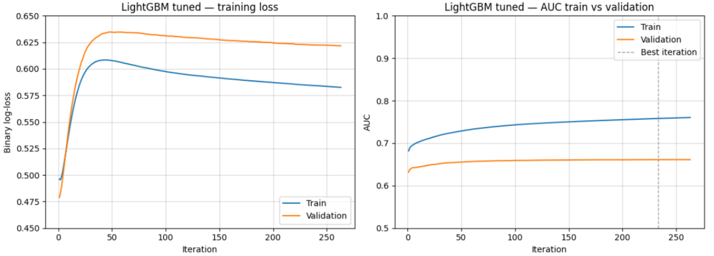
Fig. 4: LightGBM tuned: training/validation binary log-loss (left) and AUC (right) per boosting iteration.
