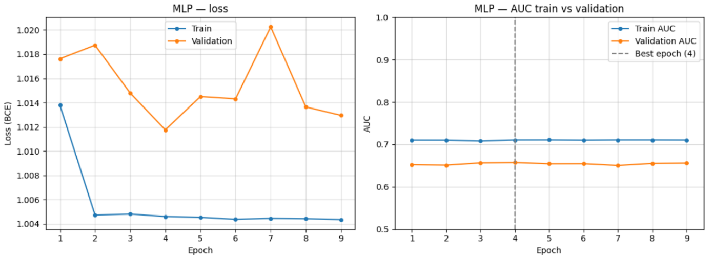
Fig. 2: MLP: training/validation loss (left) and AUC (right) per epoch.
