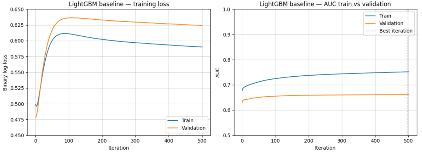
Fig. 3: LightGBM baseline: training/validation binary log-loss (left) and AUC (right) per boosting iteration.
