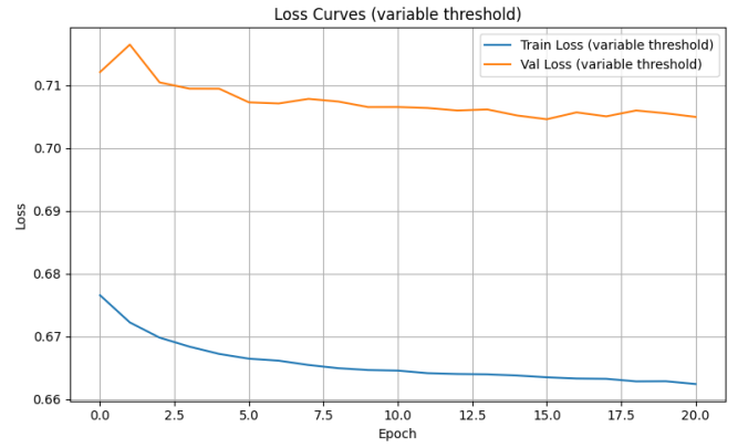
(b) LSTM+MLP
