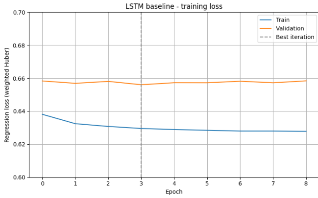
(a) LSTM baseline
