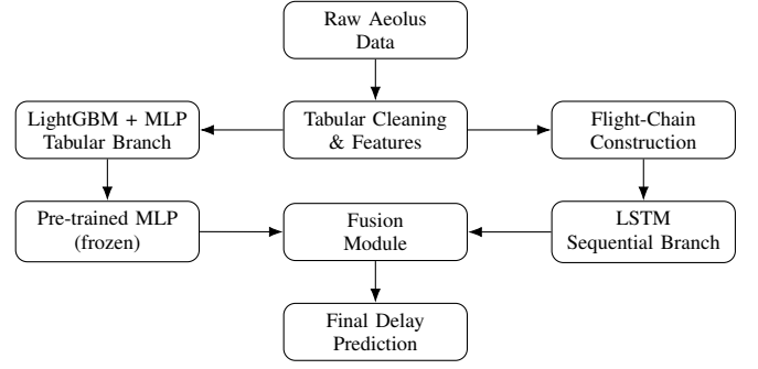
Fig. 1: Overview of the proposed flight delay prediction framework.
