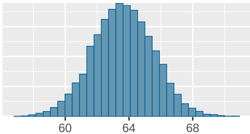
b_Intercept
