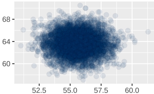
sigma
