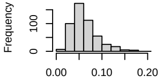
Estimate of lower CI endpoint
