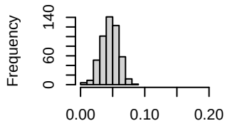
Estimate of lower CI endpoint
