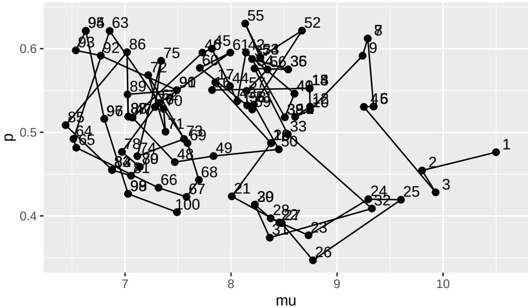
Trace plot of first 100 steps
