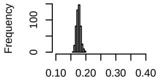
delta=0.1
