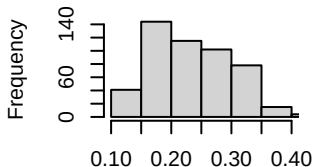
delta=0.01
