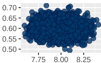
sigma
