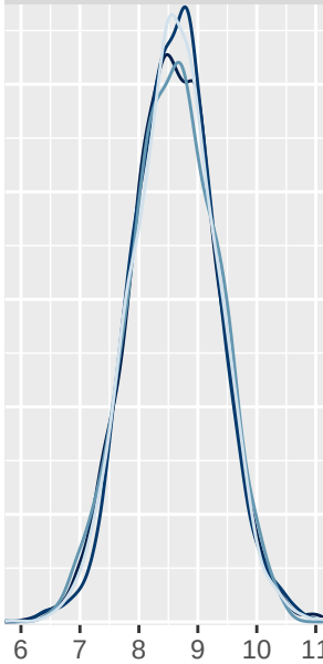
b_Intercept
