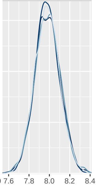
sigma
