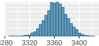
b_Intercept
