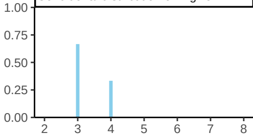
Conditional distribution of X given Y = 2
