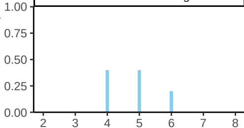
Conditional distribution of X given Y = 3
