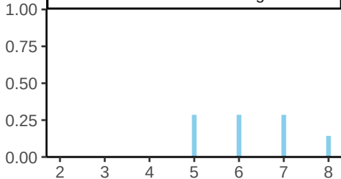
Conditional distribution of X given Y = 4
