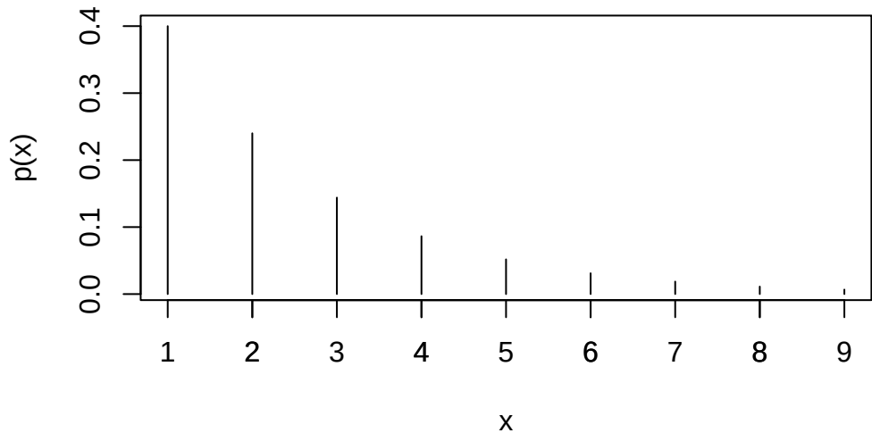
Geometric(0.4) pmf
