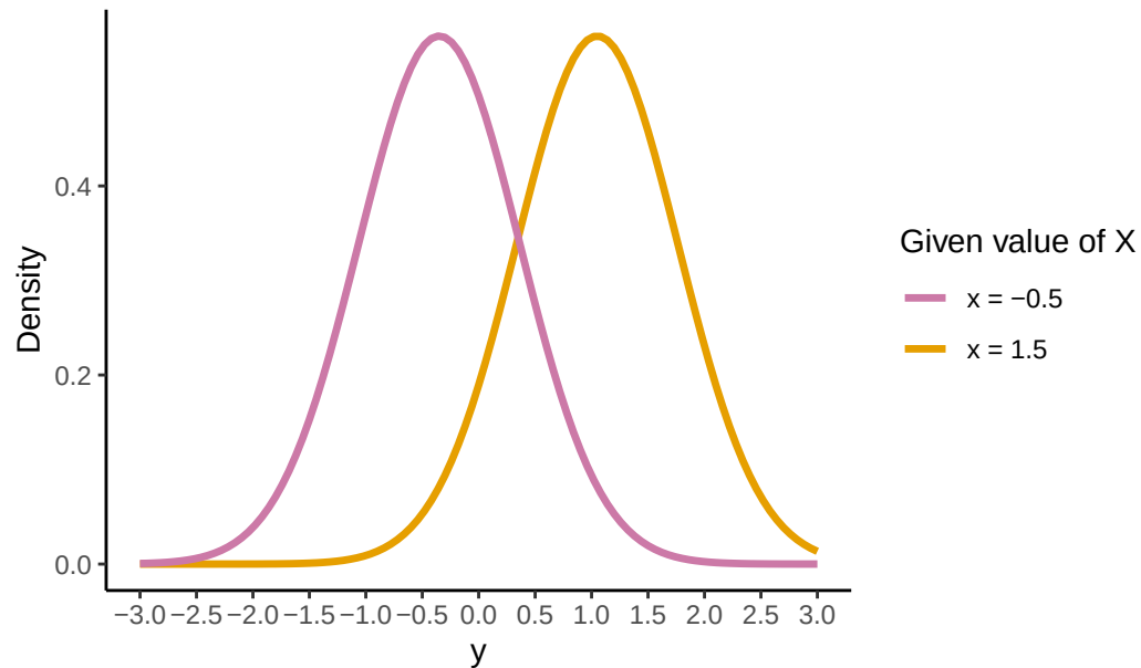
Conditional densities of Y given X = x
