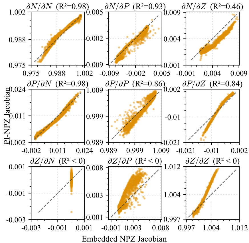
Embedded NPZ Constraints vs PI-NPZ
