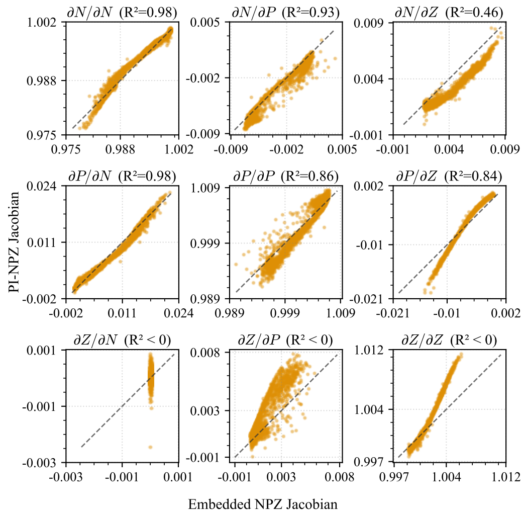
(b) Embedded NPZ Constraints vs PI-NPZ
