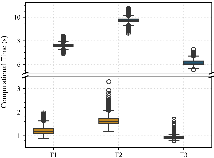
(a) 4D-Var Computational Time
