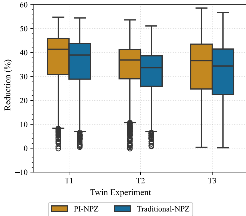
(b) Cost Function Reduction
