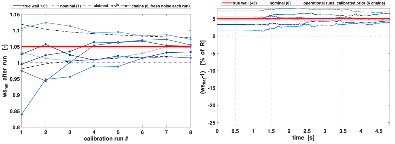
Config 5 — \bar{w}_s as a calibration constant: sequential posterior handoff (run n 's (\hat{w}_s, \sqrt{P_{w_s}}) = run n+1 's prior), 6 chains \times 8 runs, fresh noise each run, true wall 1.05 (left); operational run on the calibrated prior — cross-chain \hat{w}_s error std 1.3%, descent peak 1.69% ( \approx the config-1 locked floor) (right).
