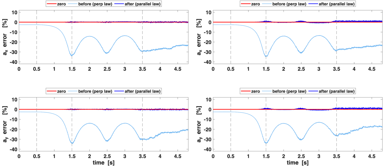
Config 6 — Stage 1a, x/y gain estimation before (perpendicular law, b=9/8 ) vs after (derived parallel law, S1 parallel block): 6-seed means desc 34.8/34.1 \rightarrow 0.92/0.86\% , hold -25.0/-22.6 \rightarrow -0.04/+0.01\% ; z bit-identical. Seed 7 (left) vs seed 11 (right).
