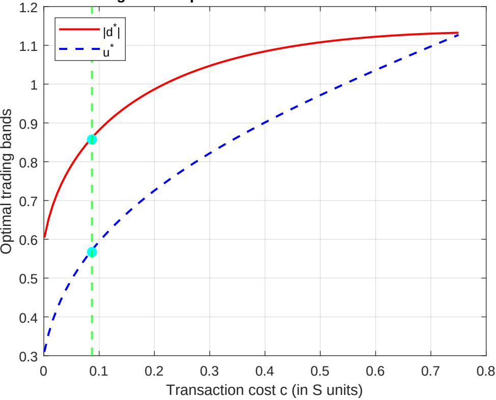
Figure 3 – Optimal bands vs. transaction cost
