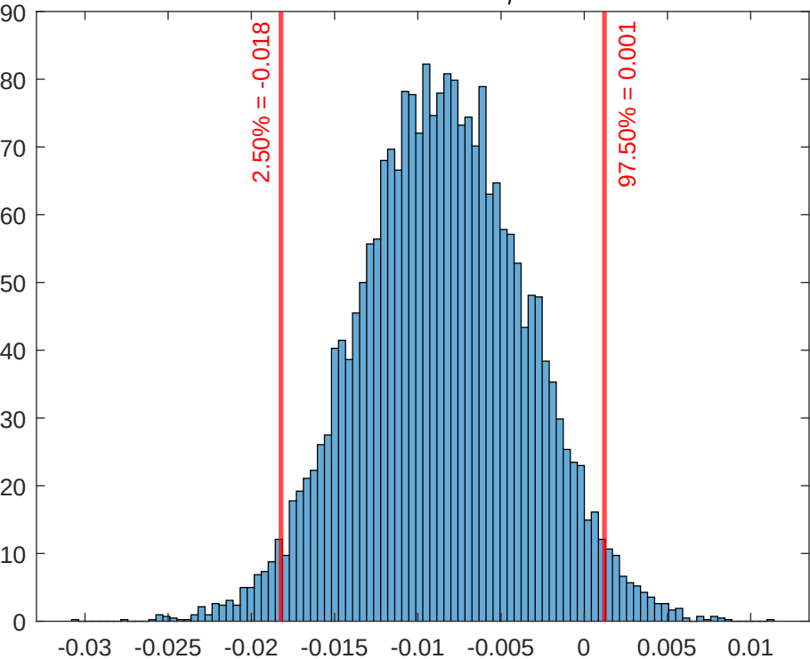
Distribution of \hat{\eta}
