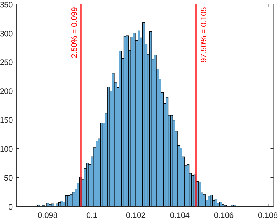
Distribution of \hat{\sigma}
