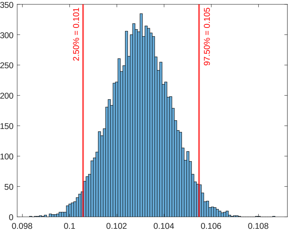
Distribution of \hat{\sigma}
