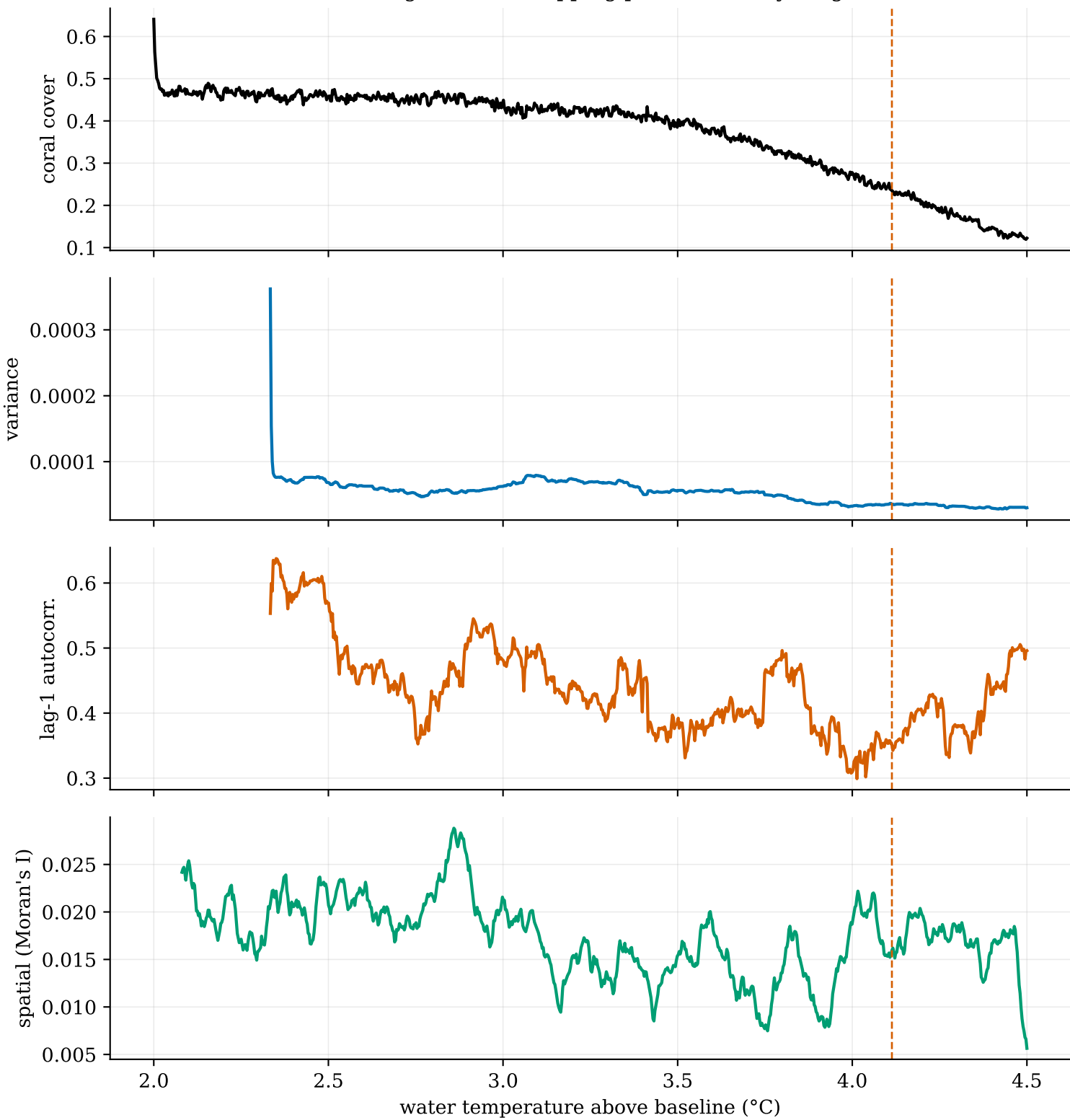
Slow warming across the tipping point: does anything warn?
