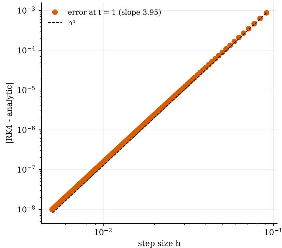
Error falls as h^4 , as it should
