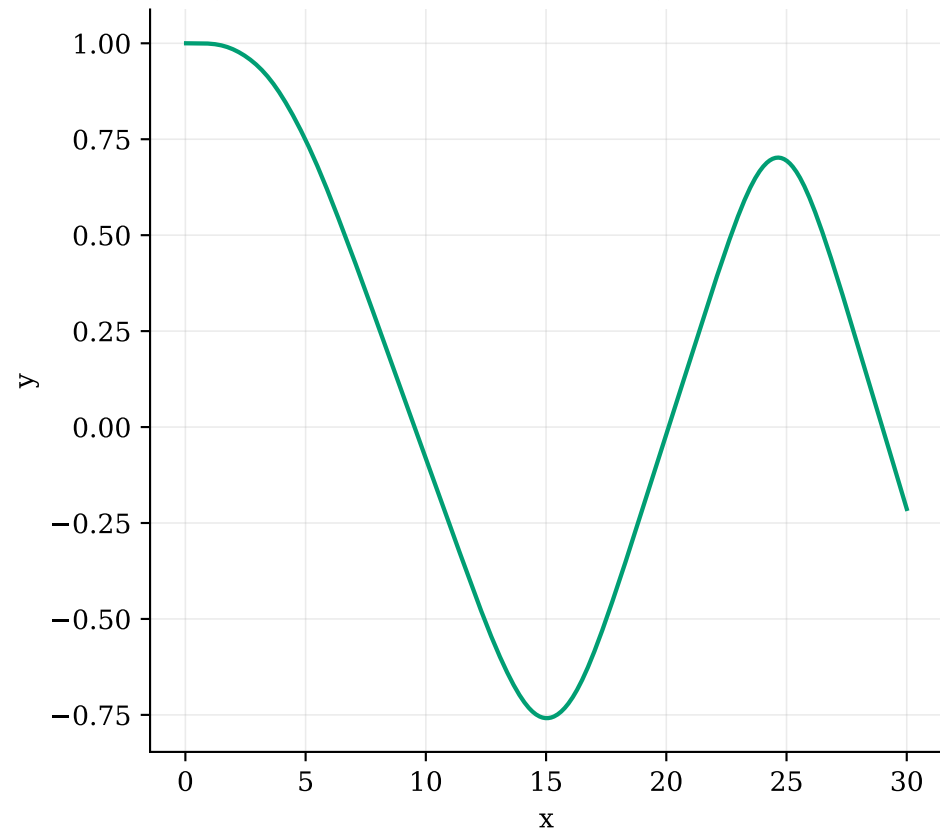
A higher-order ODE, solved as a system
