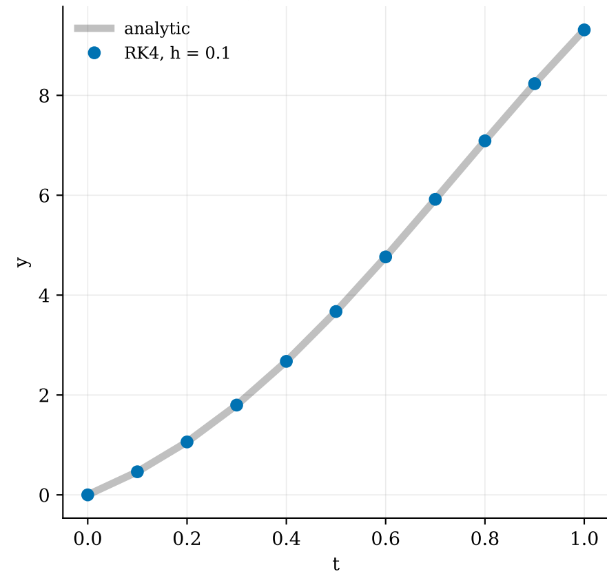
Fourth-order Runge-Kutta
