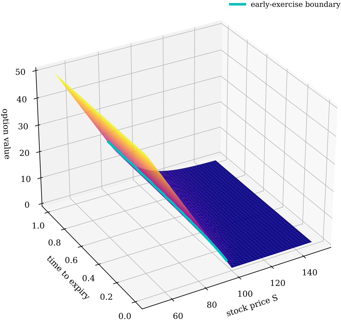
American put: Crank-Nicolson + projected SOR
